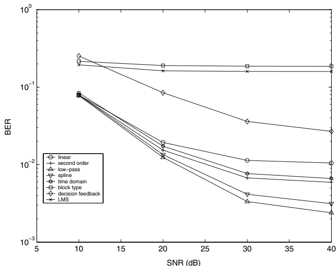
Fig. 3. 16QAM Modulation with Rayleigh Fading (Channel 1, Doppler Freq. 70Hz)
