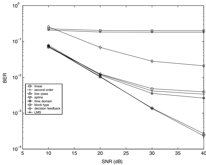
Fig. 6. 16QAM Modulation with Rayleigh Fading (Channel 2, Doppler Freq. 70Hz)
