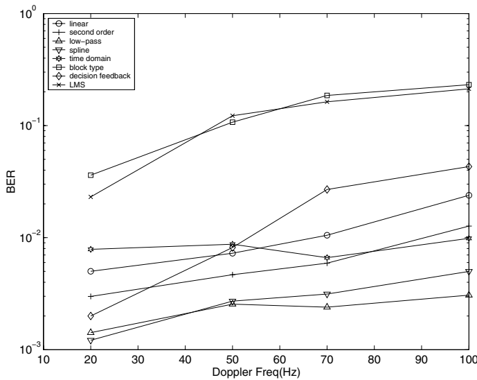
Fig. 7. 16QAM Modulation with Rayleigh Fading (Channel 1, SNR 40dB)
