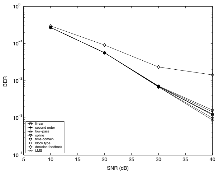
Fig. 4. DQPSK Modulation with Rayleigh Fading (Channel 1, Doppler Freq. 70Hz)
