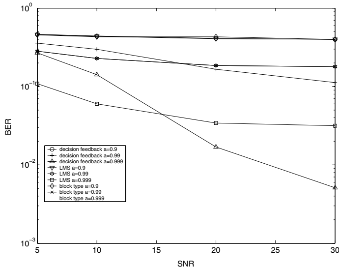
Fig. 5. 16QAM Modulation with AR Fading (Channel 1)
