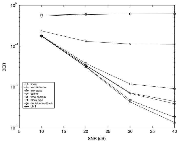
Fig. 2. QPSK Modulation with Rayleigh Fading (Channel 1, Doppler Freq. 70Hz)
